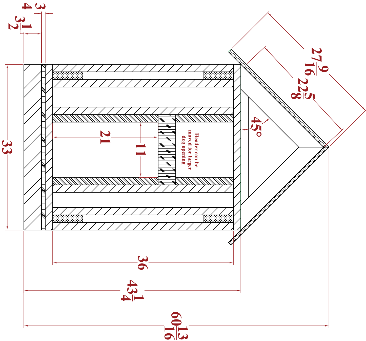
Front Wall
